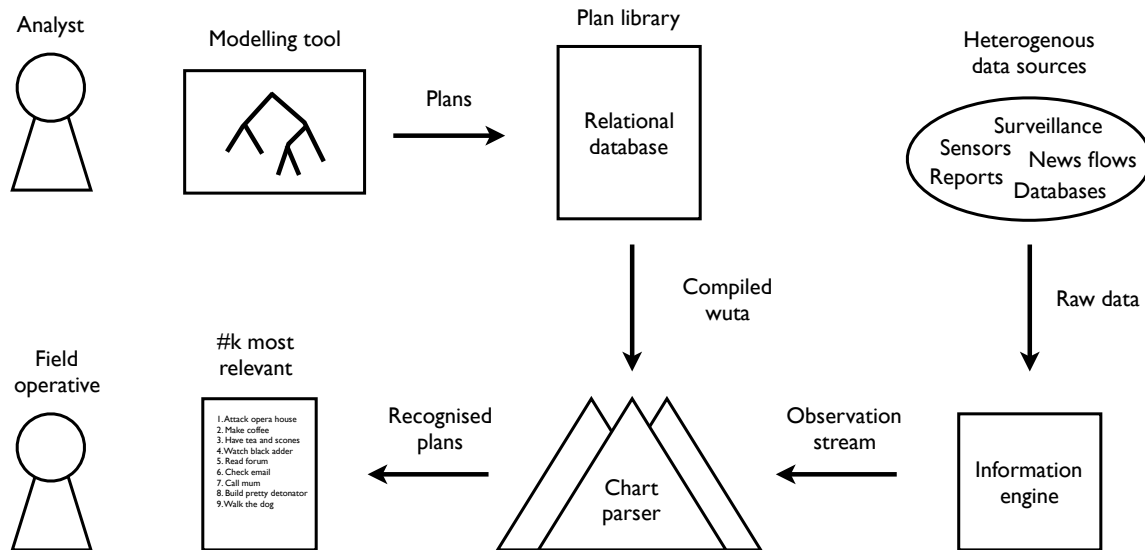
Figure 2: The user works with a modeling tool to create and edit plans. The plans are stored in a plan library and compiled upon demand into a wuta. The wuta can be used to parse observations streams and produce a list of the k plans that are most likely to be active in a given moment.
